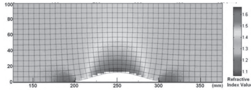
Figure 10.36. Metamaterial refractive index distribution in the ground plane cloak. The mesh lines indicate the quasi-conformal mapping. (From ref. [77], courtesy of Professor David Smith.) See color plates section.
