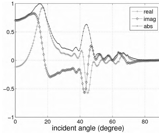
Figure 5.19. Transmission coefficient for a plane wave incident on the flat lens shown in Fig. 5.13.
