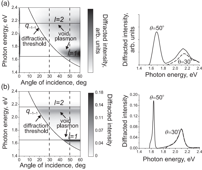
Figure 2.8. Intensity of the the first-order diffracted beam as a function of photon energy \hbar\omega and angle of incidence \theta (a) measured from and (b) calculated for a surface of nanoporous gold. The right-hand panels show the measured and calculated spectra corresponding to two angles of incidence, 30^\circ (dashed) and 50^\circ (solid), marked by dashed vertical lines in the contour maps.
