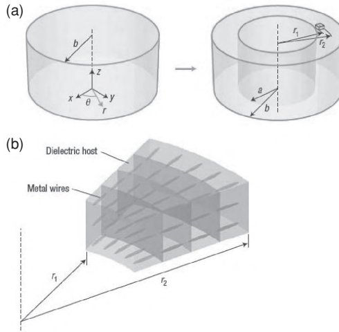
Figure 10.18. Coordinate transformation and structure of the nonmagnetic optical cloak. (a) The coordinate transformation that compresses a cylindrical region r , b into a concentric cylindrical shell a , r , b . There is no variation along the z direction; r_1 and r_2 define the internal and external radius of a fraction of the cylindrical cloak. (b) A small fraction of the cylindrical cloak. The wires are all perpendicular to the cylinder's inner and outer interfaces, but their spatial positions do not have to be periodic, and can be random. Also, for large cloaks, the wires can be broken into smaller pieces that are smaller in size than the wavelength.
