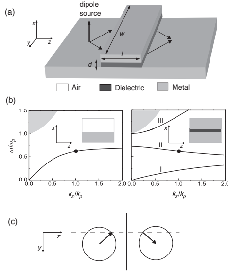
Figure 8.3. (a) Geometry of an imaging system consisting of a stripe of a metal–dielectric–metal (MDM) structure on a metal surface. The arrows on the metal surface indicate the lens operation. (b) Dispersion relations for modes of a metal–air interface (left panel), and for modes in an MDM structure with d = 0.1\lambda_p and \varepsilon_d = 4 (right panel). The corresponding structures are shown in the insets of the respective panels. The gray areas represent the continuum of extended modes in the metal regions. The black dots in both panels indicate the frequency \omega_0 at which the wave numbers match in magnitude. (c) The constant-frequency contour at \omega_0 for both the metal surface region (left side) and the MDM region (right side). Arrows indicate group velocity direction. Dashed line represents conservation of parallel wave vector.
