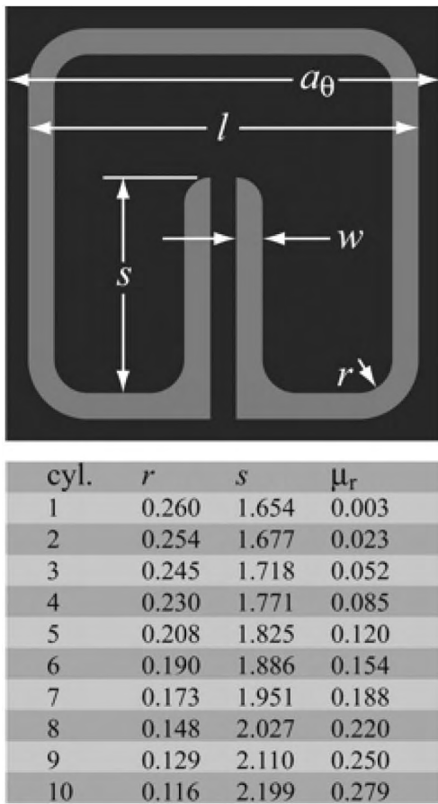
Figure 10.27. Spilt ring resonator design of the microwave cloaking structure. The in-plane lattice parameters are a_\theta = a_z = 10/3 mm. The ring is square, with edge length l = 3 mm and tracewidth w = 0.2 mm. The substrate is 381- \mu\text{m} -thick Duroid 5870 ( \epsilon = 2.33 , t_d = 0.0012 at 10 GHz, where t_d is the loss tangent). The Cu film, from which the SRRs are patterned, is 17 \mu\text{m} thick. The parameters r and s are given in the table together with the associated value of \mu_r . The extractions gave roughly constant values for the imaginary parts of the material parameters, yielding 0.002 and 0.006 for the imaginary part of \epsilon_z and \mu_r , respectively. The inner cylinder (cyl.) is 1 and the outer cylinder is 10. (From ref. [58], courtesy of Professor David Smith.)
