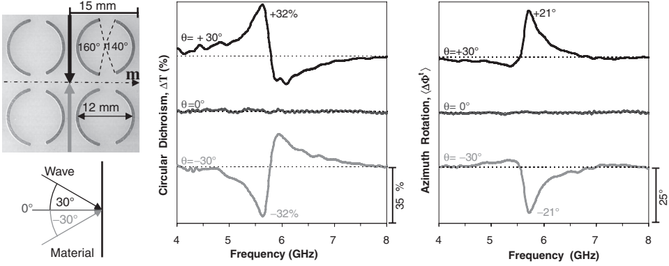
Figure 4.7. Experimental demonstration of optical activity due to extrinsic 3D chirality. Spectra of transmission circular dichroism, \Delta T , and polarization rotation, \langle \Delta \Phi' \rangle , measured for a planar metamaterial based on achiral asymmetrically split wire rings (wallpaper group pm ). The respective zero-level is indicated by a dashed line. The 3D-chiral phenomena have reversed signs for opposite angles of incidence \theta = \pm 30^\circ and vanish at normal incidence. The structure's line of mirror symmetry \mathbf{m} is oriented perpendicular to the plane of incidence ( \tilde{\varphi} = \pi/2 ), which ensures the absence of the asymmetric effect discussed in Section 4.4.2. How extrinsic 3D chirality controls the properties of this metamaterial is discussed in detail in ref. [13].
