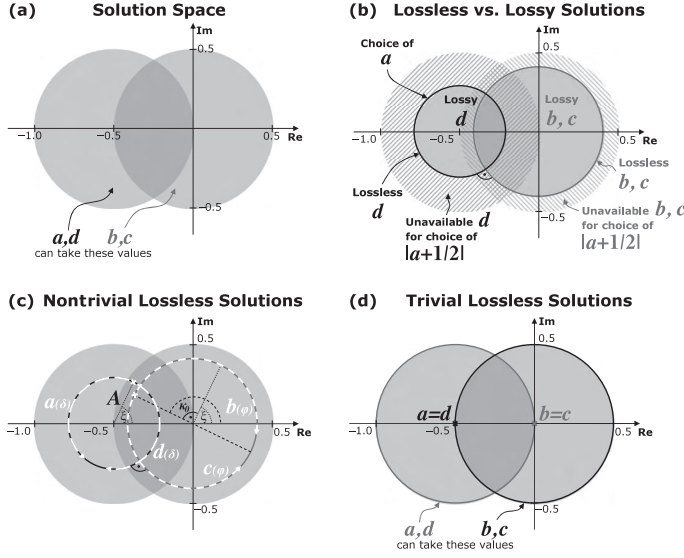
Figure 4.13. Constraints on the scattering coefficients a, b, c, d from energy conservation. (a) The solution space for a, b, c, d . (b) Lossy vs. lossless solutions for b, c, d for a particular choice of |a + 1/2| = \text{const} (here 1/\sqrt{3} ). The roles of a, d can be switched. (c) The nontrivial solutions (4.104) for the lossless case illustrated for an arbitrary choice of A, \xi . Solutions for a, d are corresponding points on the dashed arrows indicating a and d as functions of \delta . Solutions b, c are corresponding points on the dashed arrows indicating b and c as functions of the parameter \varphi . (d) Trivial solutions for the lossless case: a = d = -1/2 is shown in black (Eq. (4.105)) and b = c = 0 is plotted in gray (Eq. (4.106)).
