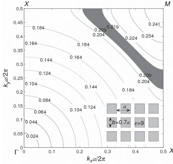
Figure 5.11. EFS of the TM modes of a square lattice PhC. The lattice is made of square rods of alumina ( \epsilon = 9 ) with a filling ratio 0.49 (see inset). The shaded area is the window of AANR for the PhC with surface grating a_s = 2a (see Fig. 5.13). A slab of this PhC is oriented such that the surface normal is along the \Gamma X direction.
