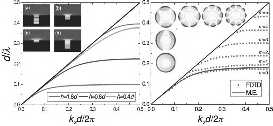
Figure 7.6. Spoof SPP dispersion relation for wires of radius R = 2d perforated with rings of width a = 0.2d . Left panel: \theta -independent bands for different ring depths. The inset shows the electric field amplitude ( r > R - h ) at the edge of the bands. Right panel: FDTD bands for higher azimuthal orders ( m ) for h = 0.5d . The insets plot the electric field patterns at the band edge ordered with increasing m from the left bottom corner to the right top corner of the figure. See color plates section.
