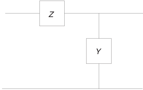
Figure 10.7. Generalized distributed impedance/admittance system.
