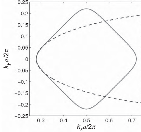
Figure 5.16. Fitting of the EFS of the TM modes at \omega a / 2\pi c = 0.219 by Eq. (5.12). Here \sigma_0 = 4 and \kappa a / 2\pi c = 1.16 . Note that the center of the EFS is shifted from the M point to the X point due to the surface grating with a_s = 2a .
